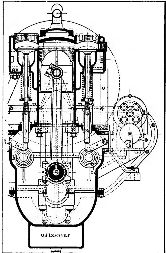
Fig. 6—Transverse section of the third cylinder of the motor
